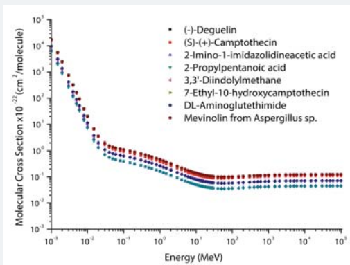
Figure 2: Molecular cross sections of selected enzyme inhibitors versus photon energy.
