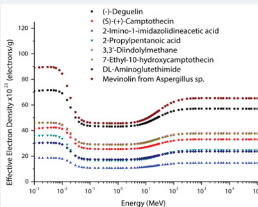
Figure 6: Effective electron densities of selected enzyme inhibitors versus photon energy.
