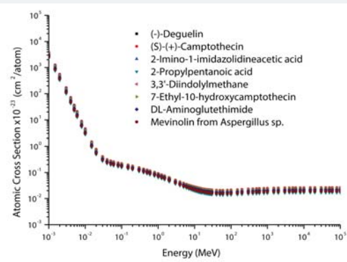
Figure 3: Atomic cross sections of selected enzyme inhibitors versus photon energy.
