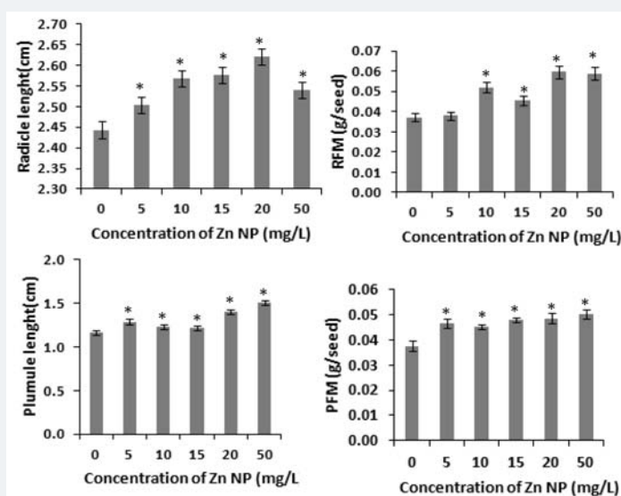
Figure 1: Effect of Zn NP on length and fresh mass of radicle and plumule of germinating rice seeds. Data presented are mean \pm SE. * indicate significant mean difference from control by LSD test ( p < 0.05 ).
